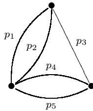
FIGURE 1. A relativistic spin network
